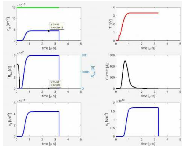
Figure 3 Saha's ionization equation calculation result
