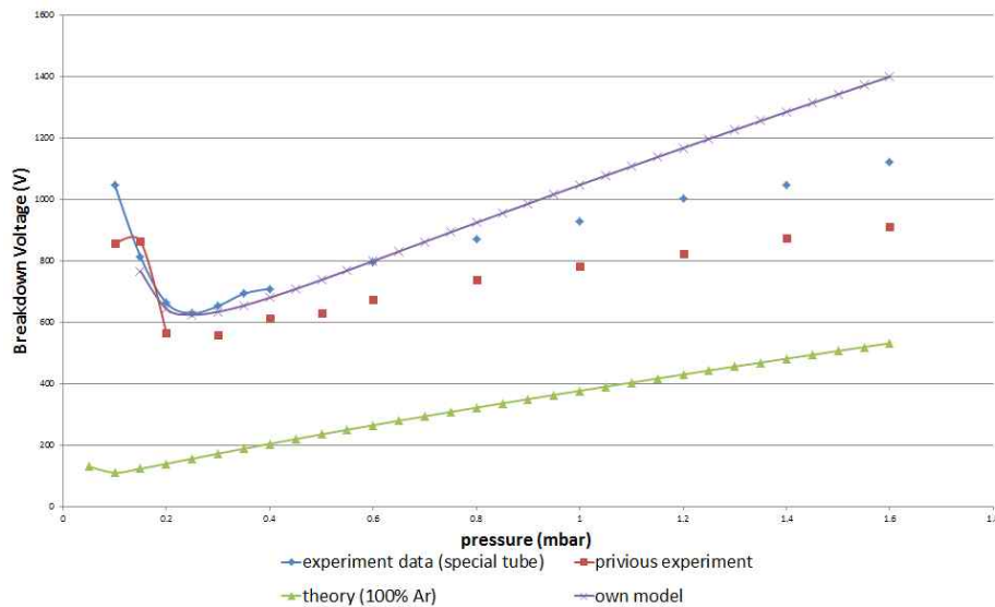
Figure 2 Paschen's curve result
