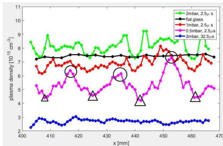
Figure 4 plasma density measurement
