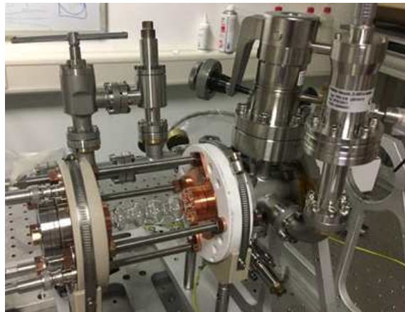
Figure 1 Overall of Plasma cell assembly
